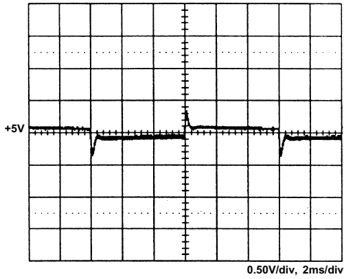
+5V step from 4A to 20A
